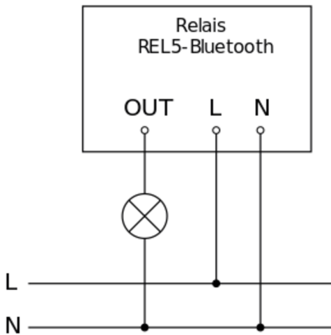
Circuit diagram 1
